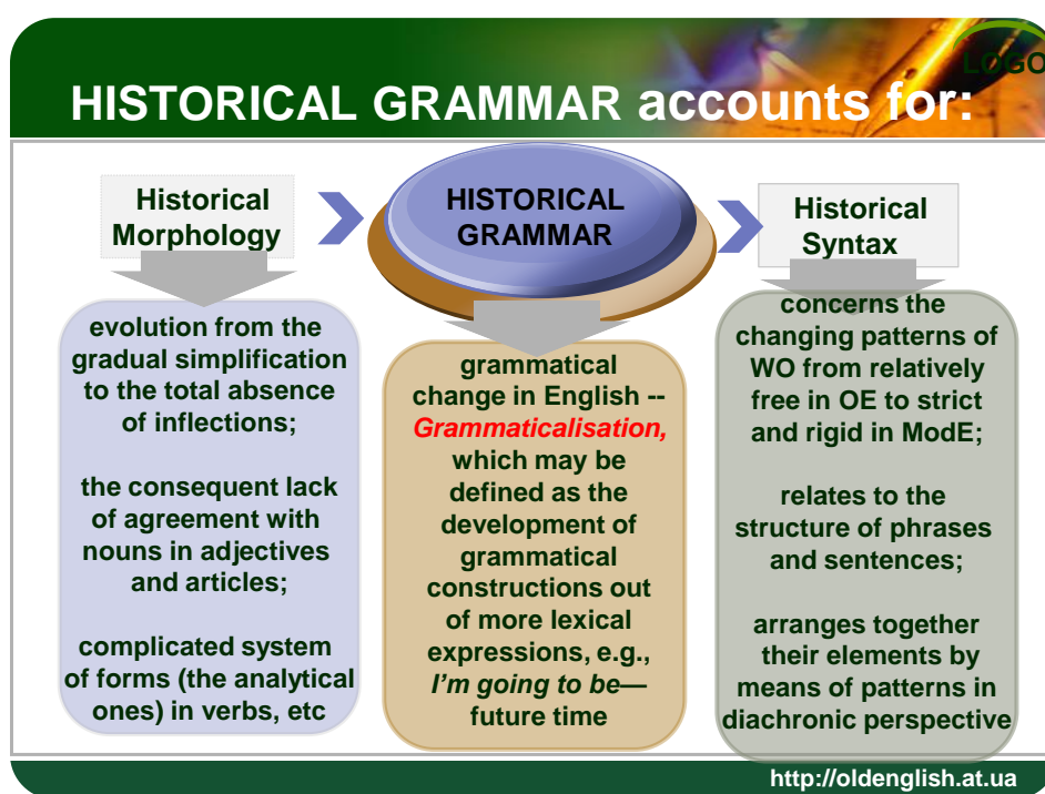
Figure 1.10. Historical grammar accounts for the morphological and syntactical changes of language across time
