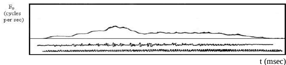
Fig. 1.7. The electro-kymogram of the English word name [næm]
