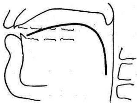
Fig. 2.52. Tongue-position of English [ə] at the end of a word
