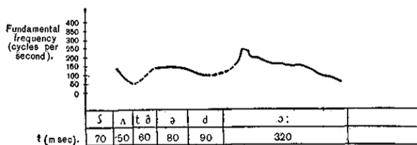
Fig. 9.4. Shut the door! (command). [ 'ʃʌt ðə .dɔ: ||]
