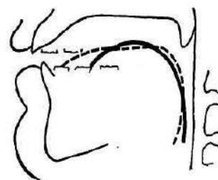
Fig. 2.41. Tongue-position: English [ʌ] _____ English [ɑ:] - - - - -
