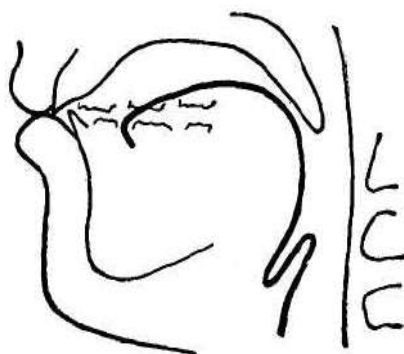
Fig. 3.7. Tongue-position of Ukrainian [M]
