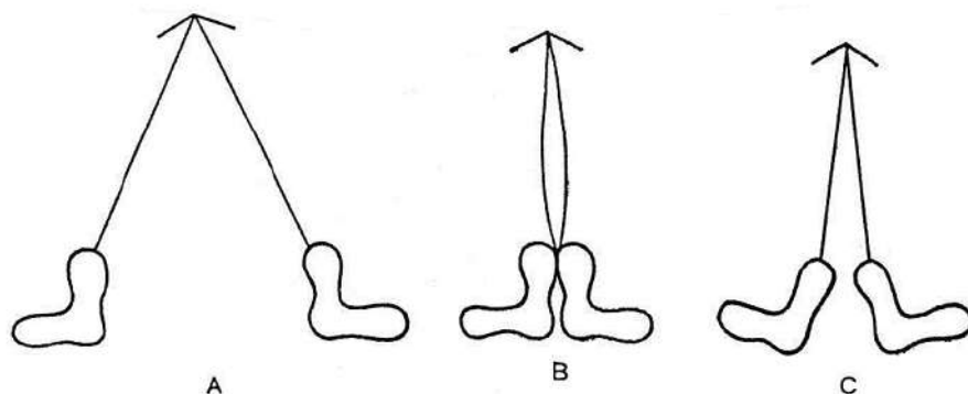
Fig. 1.19. The position of the vocal chords
