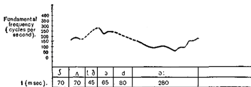
Fig. 9.5. Shut the door. (request)
