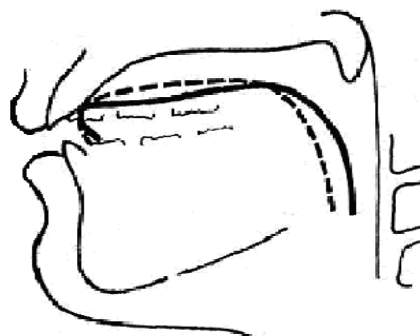
Fig. 3.36. Tongue-position: English clear [l] ————— English dark [l] - - - - -
