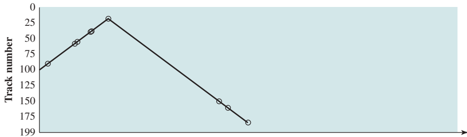
(b) SSTF
