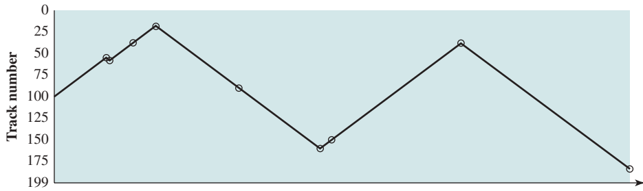
(a) FIFO
