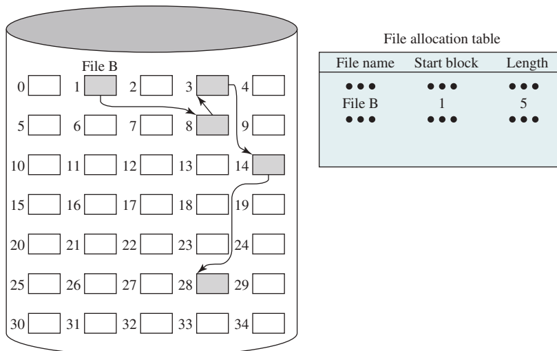
Figure 12.11 Chained Allocation
