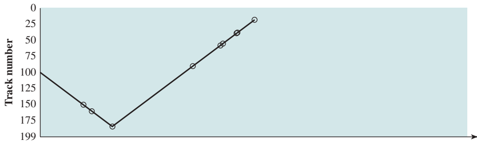
(c) SCAN
